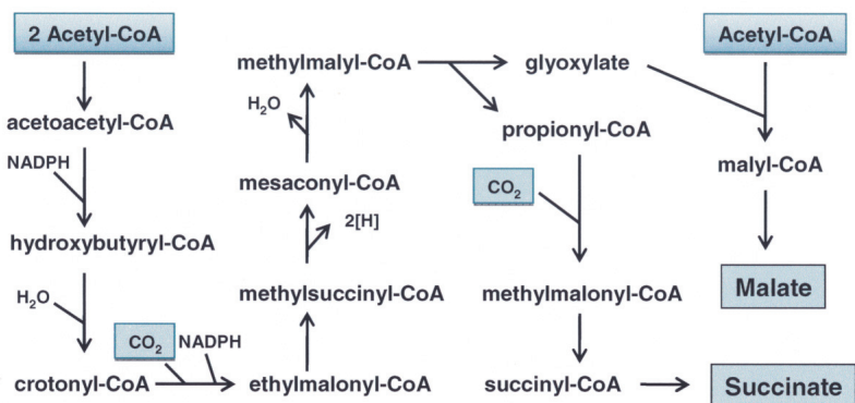
Figure 12 The ethylmalonyl-CoA (EMC) pathway for acetyl-CoA assimilation in Rhodospirillum rubrum , presented in a convenient form and similar layout to Figure 9. Note that there are two forms (R and S) of ethylmalonyl-CoA and two forms (R and S) of methylmalonyl-CoA (see Figure 11) which are interconverted by the same epimerase. The carbon balance of the pathway as shown here is:
