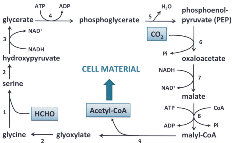
Figure 3 The serine cycle as proposed by Peel, Large, Salem and Quayle 9–11 . The enzymes are 1, serine transhydroxymethylase; 2, serine-glyoxylate aminotransferase; 3, hydroxypyruvate reductase; 4, glycinate kinase; 5, enolase; 6, PEP carboxylase; 7, malate dehydrogenase; 8, malate thiokinase; 9, malyl-CoA lyase. After the initial proposal much further enzymological and mutant evidence was subsequently accumulated to confirm this pathway 3 . Note that during biosynthesis of fatty acids and poly 3-hydroxybutyrate which use acetyl-CoA as their biosynthetic starting point, this pathway is sufficient for production of acetyl-CoA from formaldehyde plus carbon dioxide.
